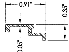
15 MEETING RAIL REINFORCEMENT
