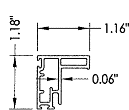
2 SASH STILE/RAIL
