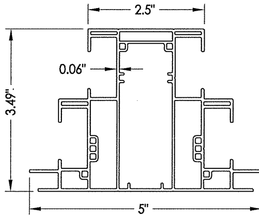
10 INTEGRAL MULLION
