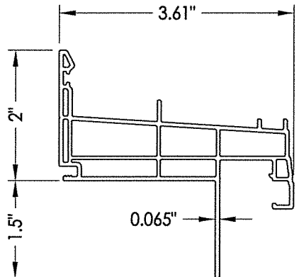
6 SILL
