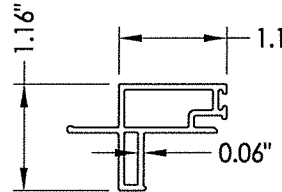
3 TOP RAIL
