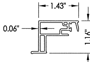
4 LOCK RAIL
